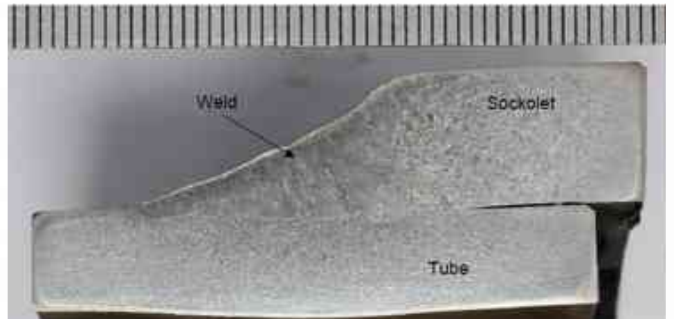
Production Weld (~2 years in Service)
